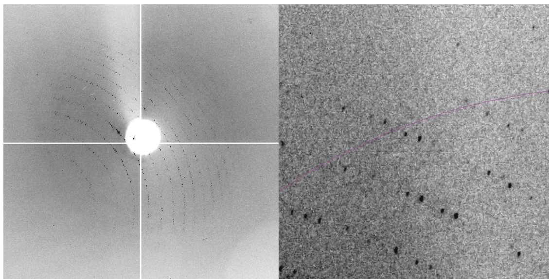
Figure 3 Diffraction image and a close-up of the highest resolution reflections. The purple line indicates 8.9 Å resolution.
